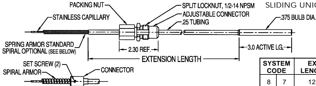
SLIDING UNION - BENDABLE EXTENSION
