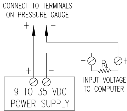
VOLTAGE/PRESSURE EXAMPLE FOR 200PSI R_L=250\Omega
